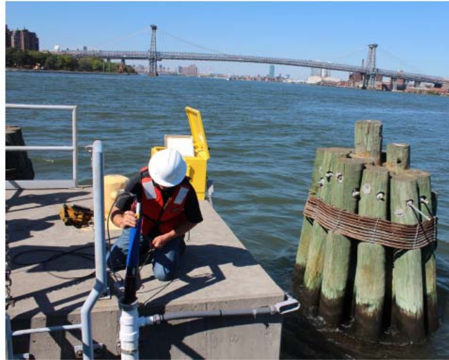
YSI EXO2 multi-parameter water quality instrument being installed by a YSI field technician at a monitoring site in New York.
